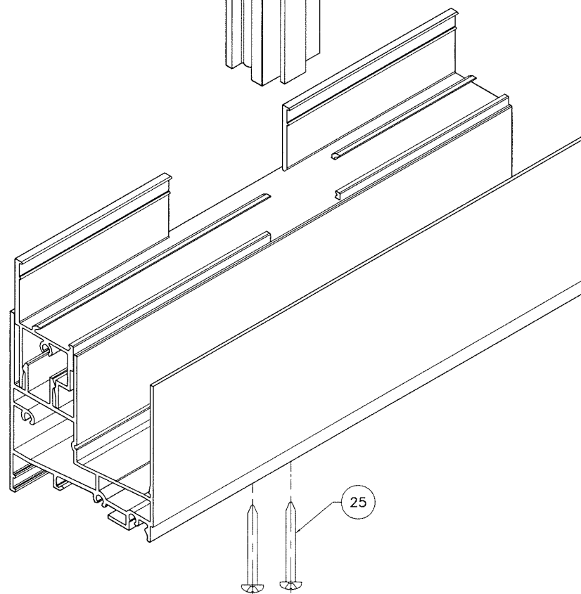
FIX. MTG. STILE TOP/BOTTOM ASSEMBLY
